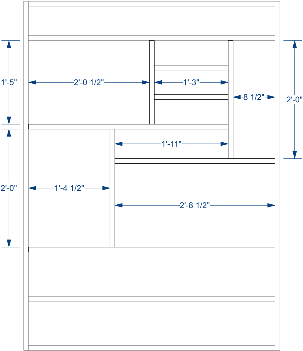
FRONT VIEW
